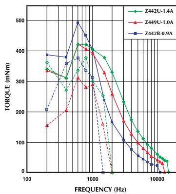
Model No: 17PY-Z442U,Z449U,Z442B Driver: Chopper Dual Supply Voltage: 24.0 (Volt)
