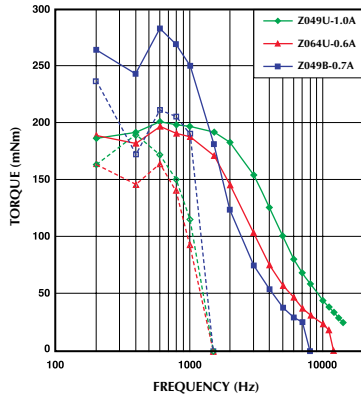
Model No: 17PY-Z049U,Z064U,Z049B Driver: Chopper Dual Supply Voltage: 24.0 (Volt)
