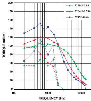
Model No: 17PY-Z249U,Z264U,Z249B Driver: Chopper Dual Supply Voltage: 24.0 (Volt)
