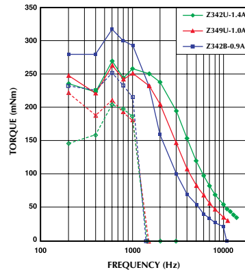
Model No: 17PY-Z342U,Z349U,Z342B Driver: Chopper Dual Supply Voltage: 24.0 (Volt)
