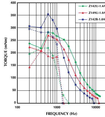
Model No: 17PY-Z142U,Z149U,Z142B Driver: Chopper Dual Supply Voltage: 24.0 (Volt)
