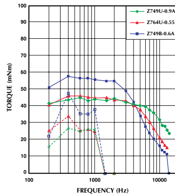
Model No: 17PY-Z749U,Z764U,Z749B Driver: Chopper Dual Supply Voltage: 24.0 (Volt)
