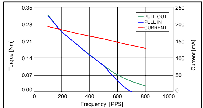
PG20S-020 Reduction Ratio 1/185.4
