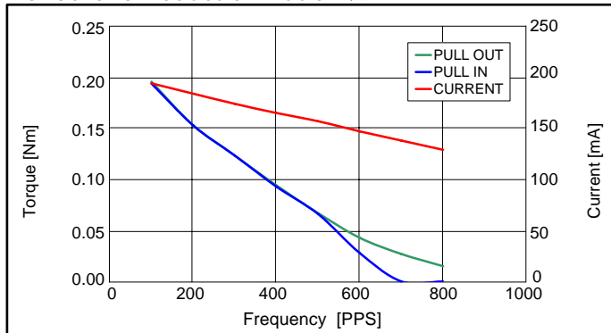
PG20S-020 Reduction Ratio 1/91
