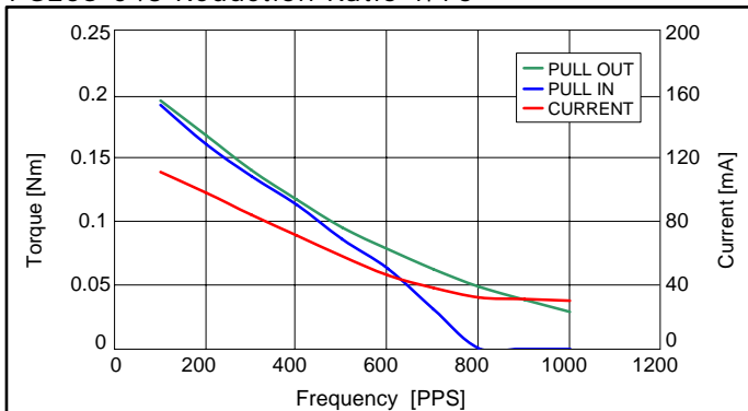
PG25S-048 Reduction Ratio 1/76
