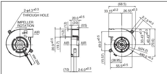
06920GA product drawing
