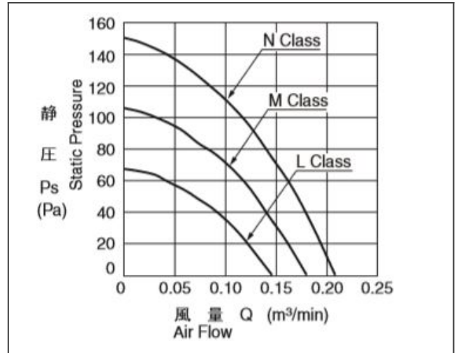
06920GA characteristic curve
