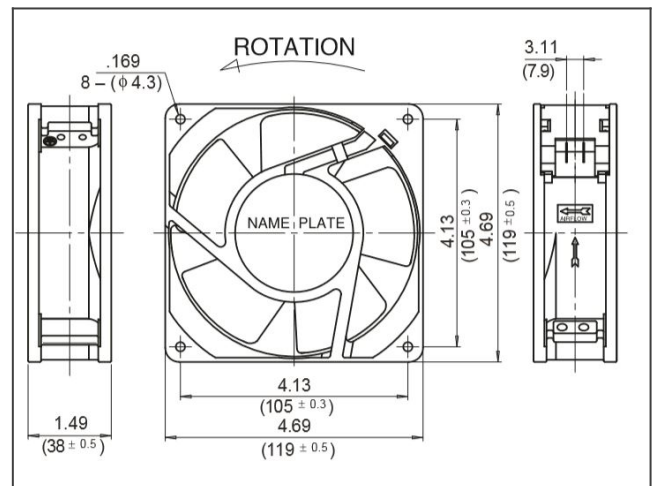
11938SB-A0N-NP plastic std product drawing
