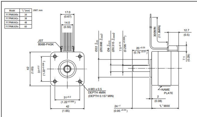
F17PMK049USTDCN product drawing
