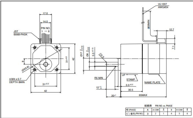
GT0036-17M000 product drawing
