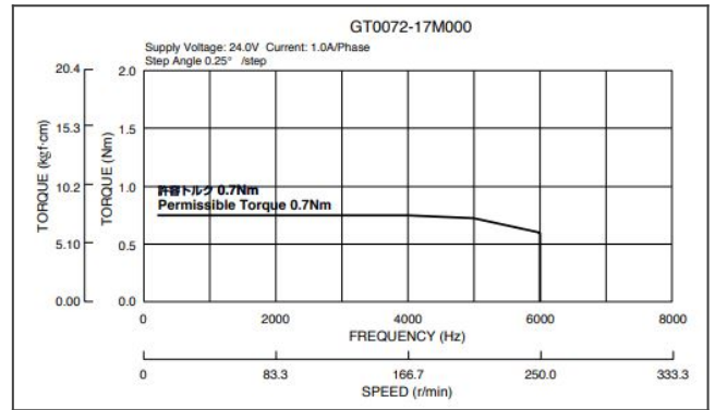
GT0072-17M000 graph
