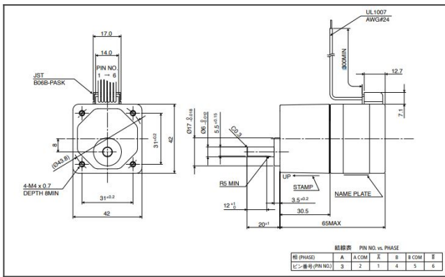
GT0072-17M000 product drawing
