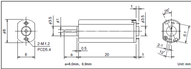
PNN13 Model Product Drawing
